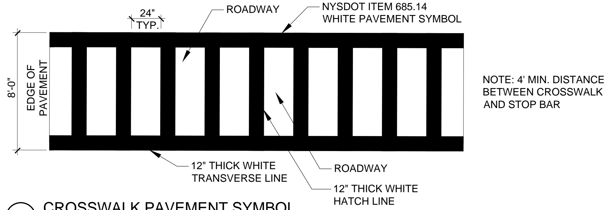
6 CROSSWALK PAVEMENT SYMBOL SCALE 1/2" = 1'-0"
