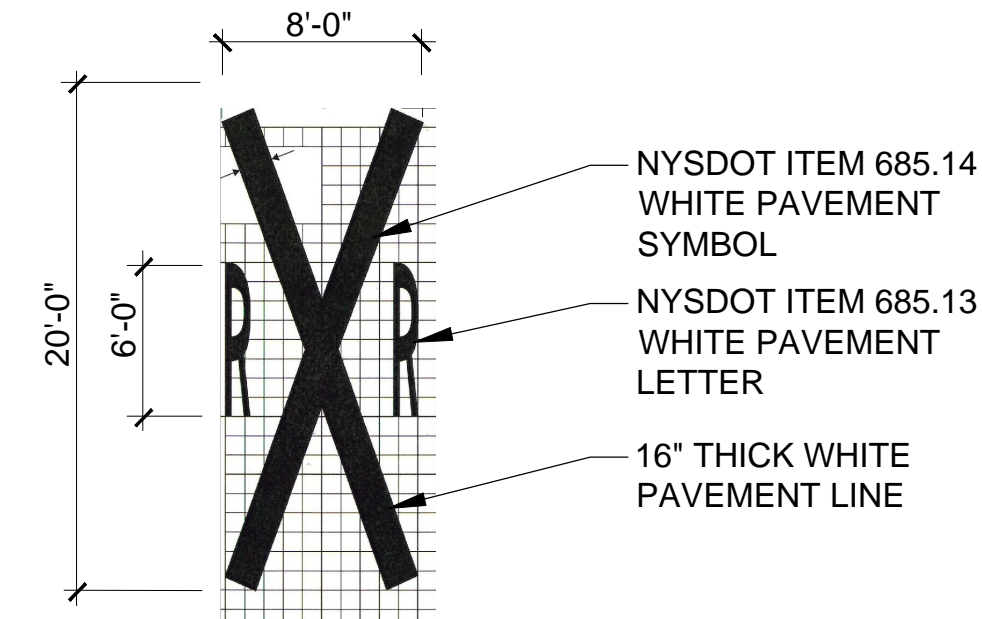
4 RAILROAD CROSSING PAVEMENT SYMBOL SCALE 1/4" = 1'-0"
