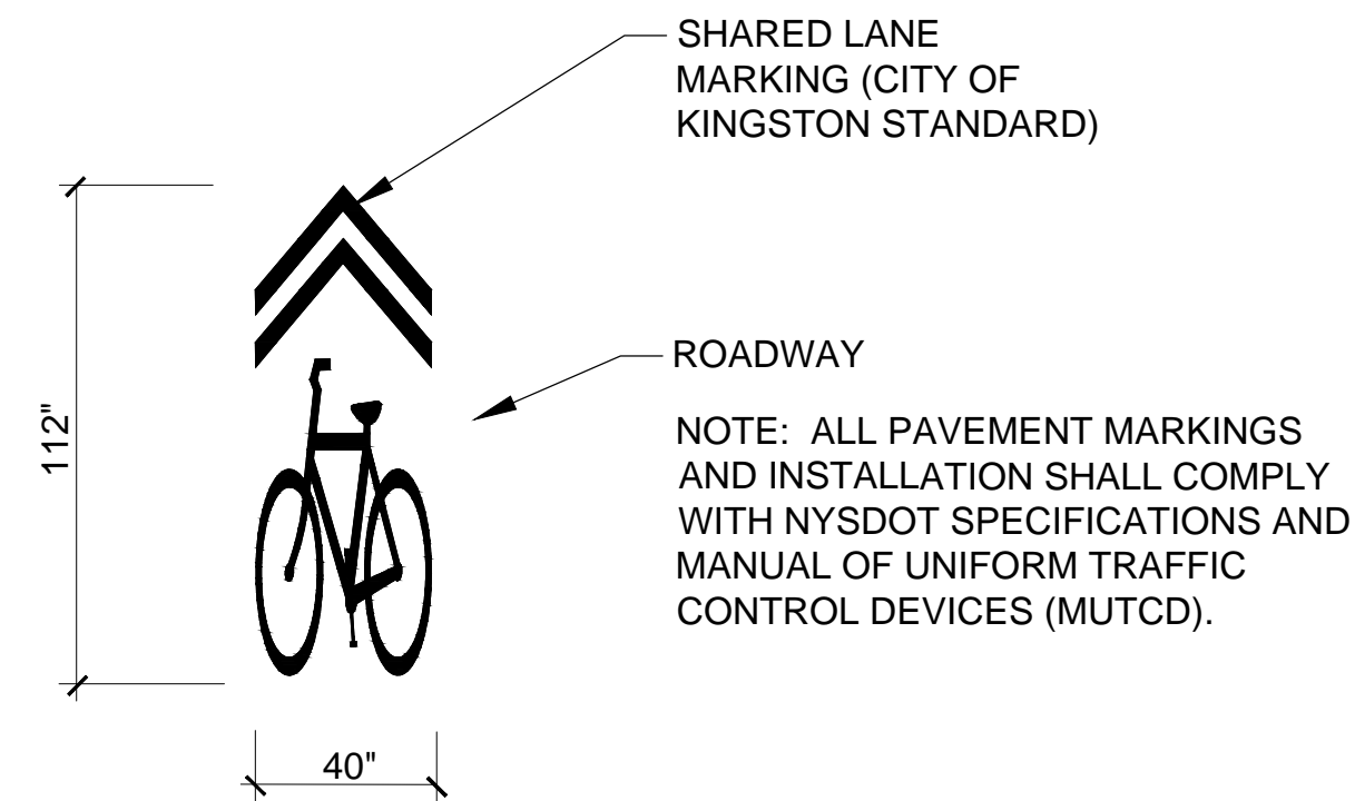
2 BIKEWAY PAVEMENT SYMBOL SCALE 1/4" = 1'-0"
