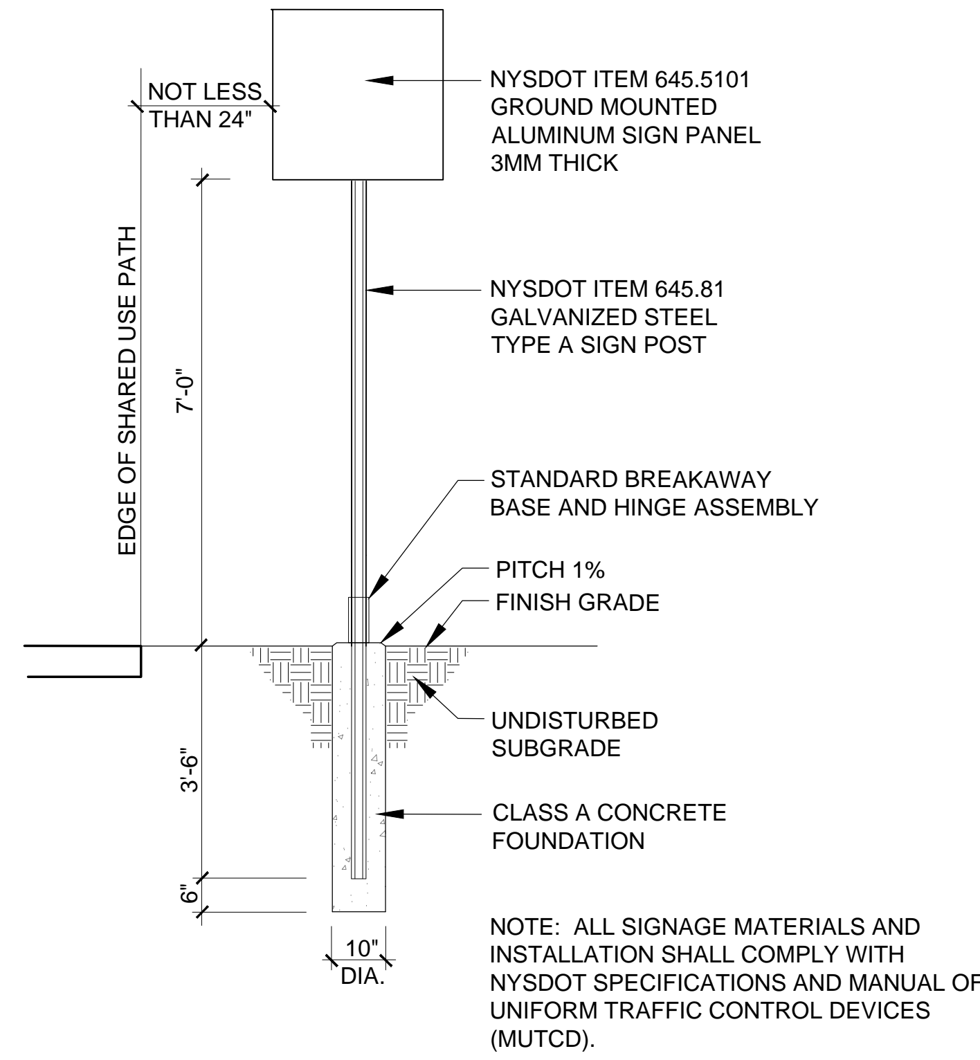
1 BIKEWAY SIGNAGE SCALE 1/2" = 1'-0"
