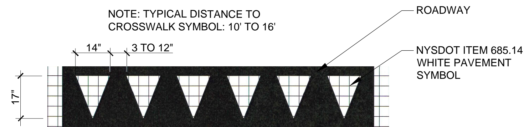
5 YIELD LINE PAVEMENT SYMBOL SCALE 1/2" = 1'-0"
