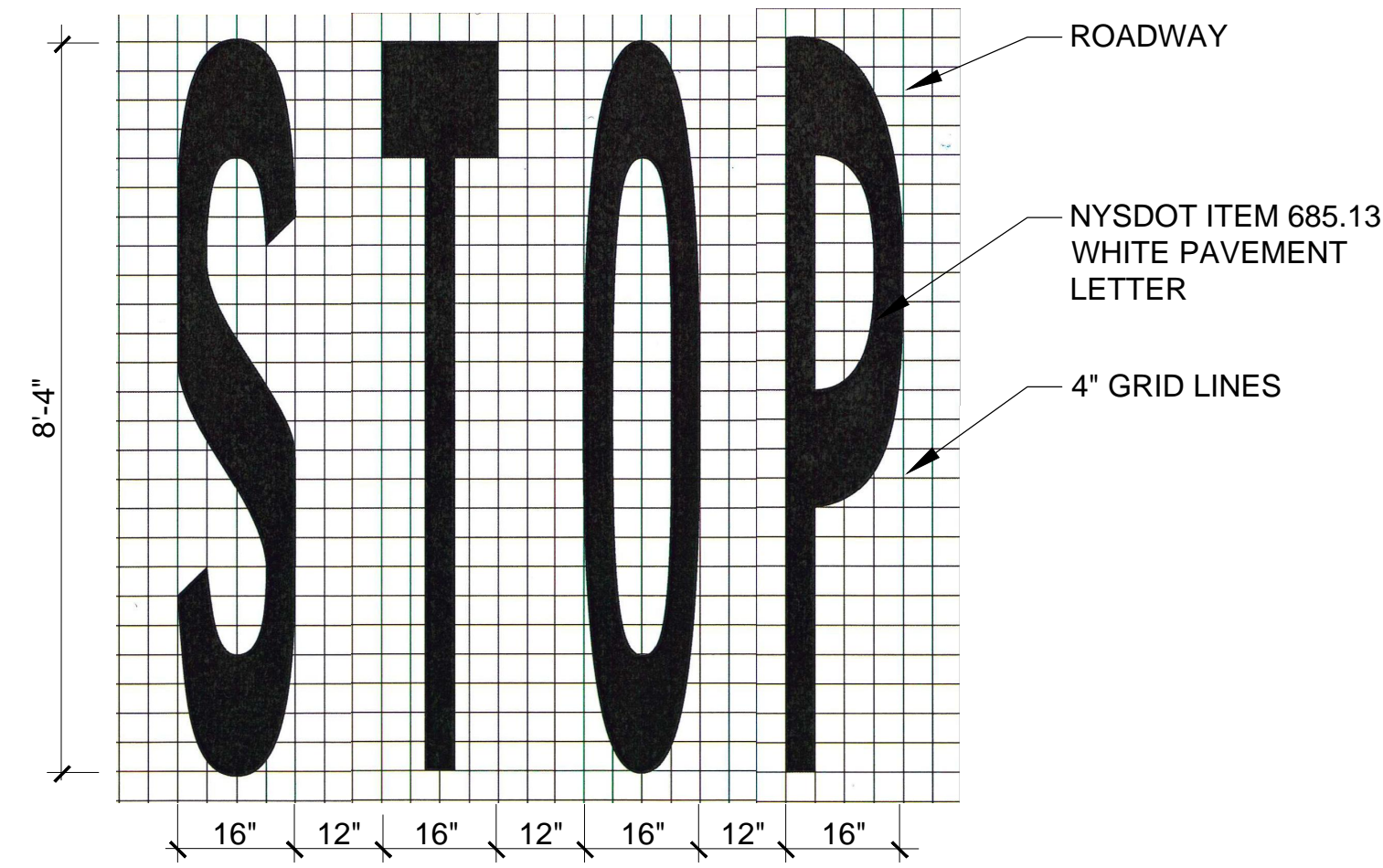
3 STOP PAVEMENT LETTERS SCALE 1/2" = 1'-0"
